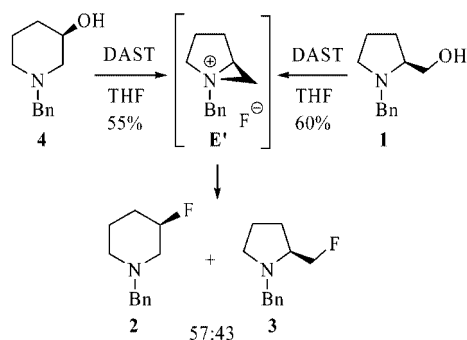
Scheme 2. Mechanism via an aziridinium intermediate.
