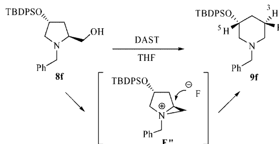
Scheme 4. Aziridinium intermediate and stereochemistry.
