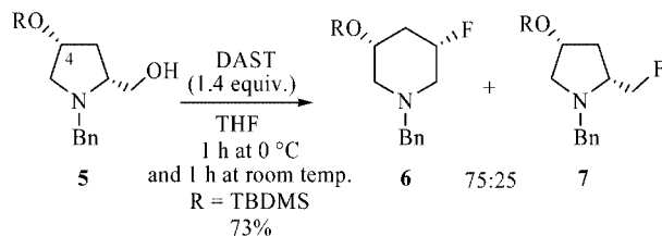
Scheme 3. Rearrangement of prolinol 5 .
